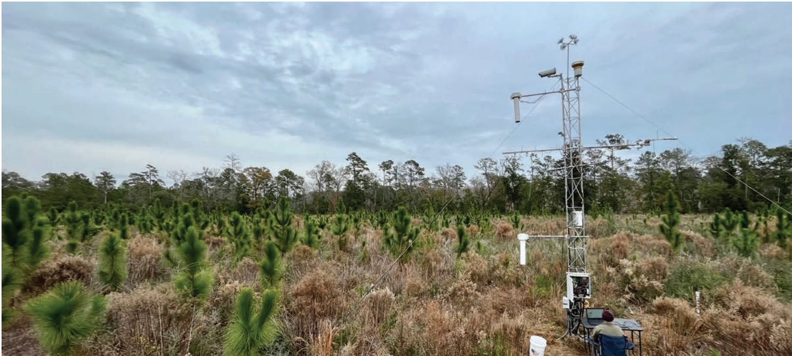
Eddy Flux tower taking atmospheric measurements to understand the role of longleaf pine forests in carbon sequestration. – Credit: Tom O’Halloran
